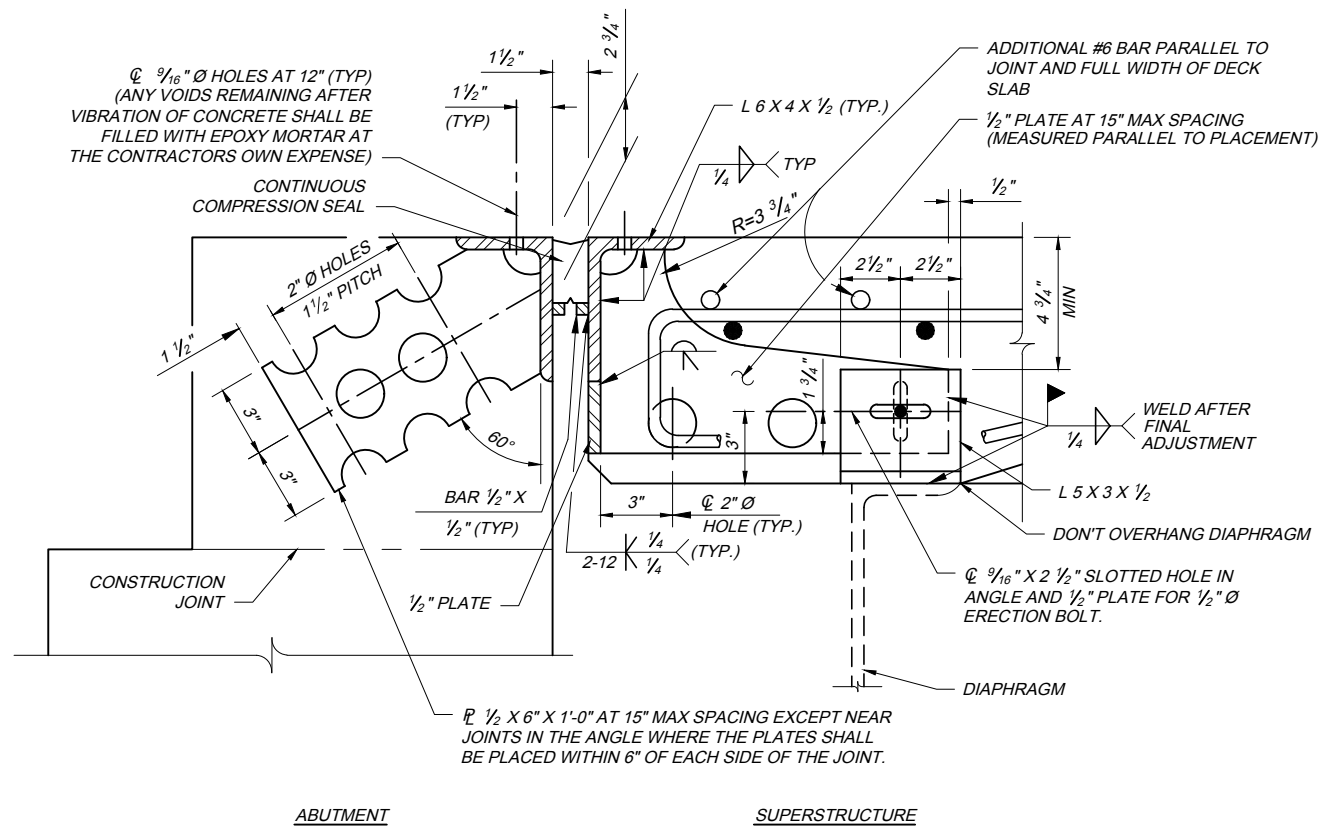
SECTION A-A (COMPRESSION SEAL)
