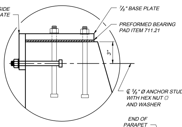
DETAIL D (POST NOT SHOWN)
