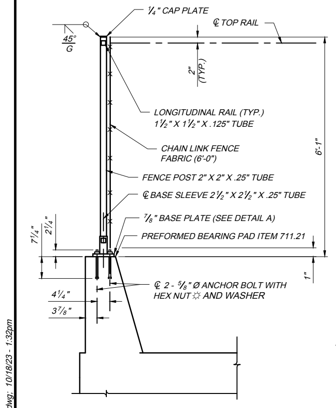
TYPE 2 CHAIN LINK FENCE DETAIL ✪ STAINLESS STEEL SELF-LOCKING HEX NUT WITH NYLON INSERT
