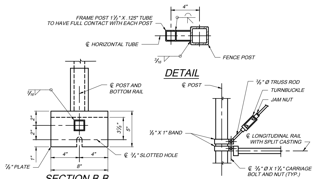
TRUSS ROD AND END PANEL RAIL ATTACHMENT
