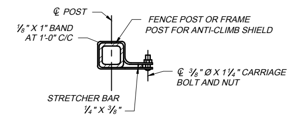
STRETCHER BAR ATTACHMENT
