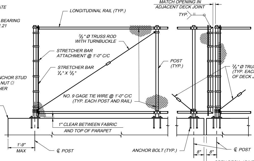
INTERIOR ELEVATION
