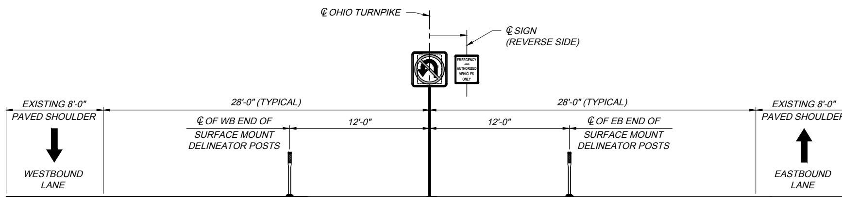
SECTION B-B
