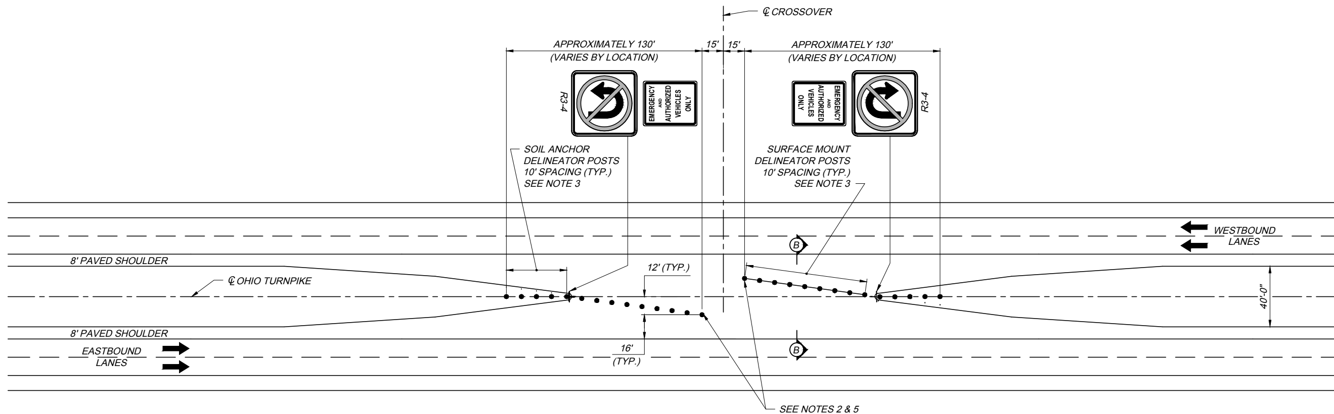
CROSSOVER DELINEATOR POST PLAN
