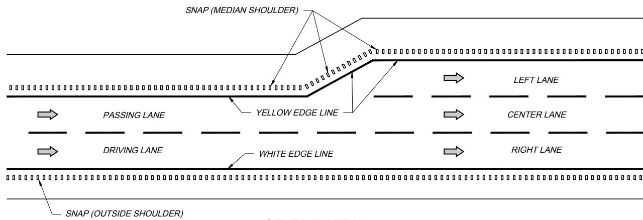
GENERAL VIEW
