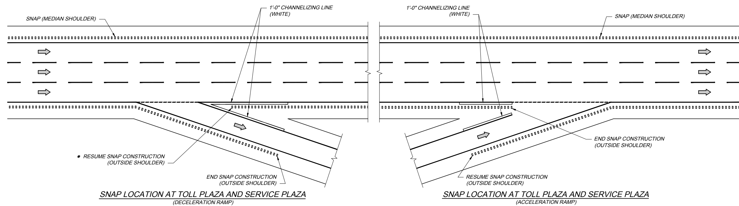
PLAN
