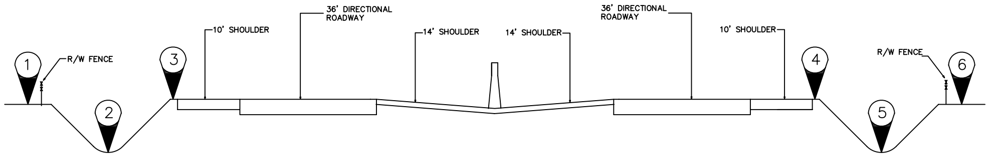
FIGURE 2 – BORING LOCATIONS 3 LANE ROADWAY
